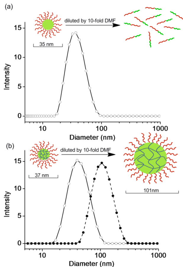
Figure 2. Distributions of hydrodynamic diameters of (a) UCL and (b) CCL micelles in water (O) before and (●) after 10-fold dilution with DMF.
